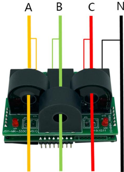
Three-phase four-wire load
